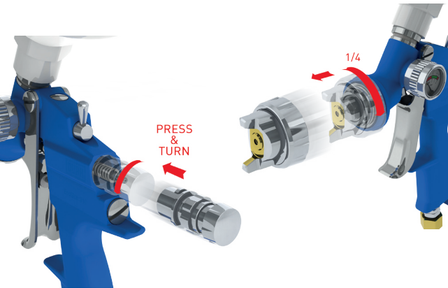
Quick & easy replacement of air cap and needle with bayonet connection.
